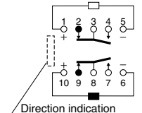
2-coil latching
